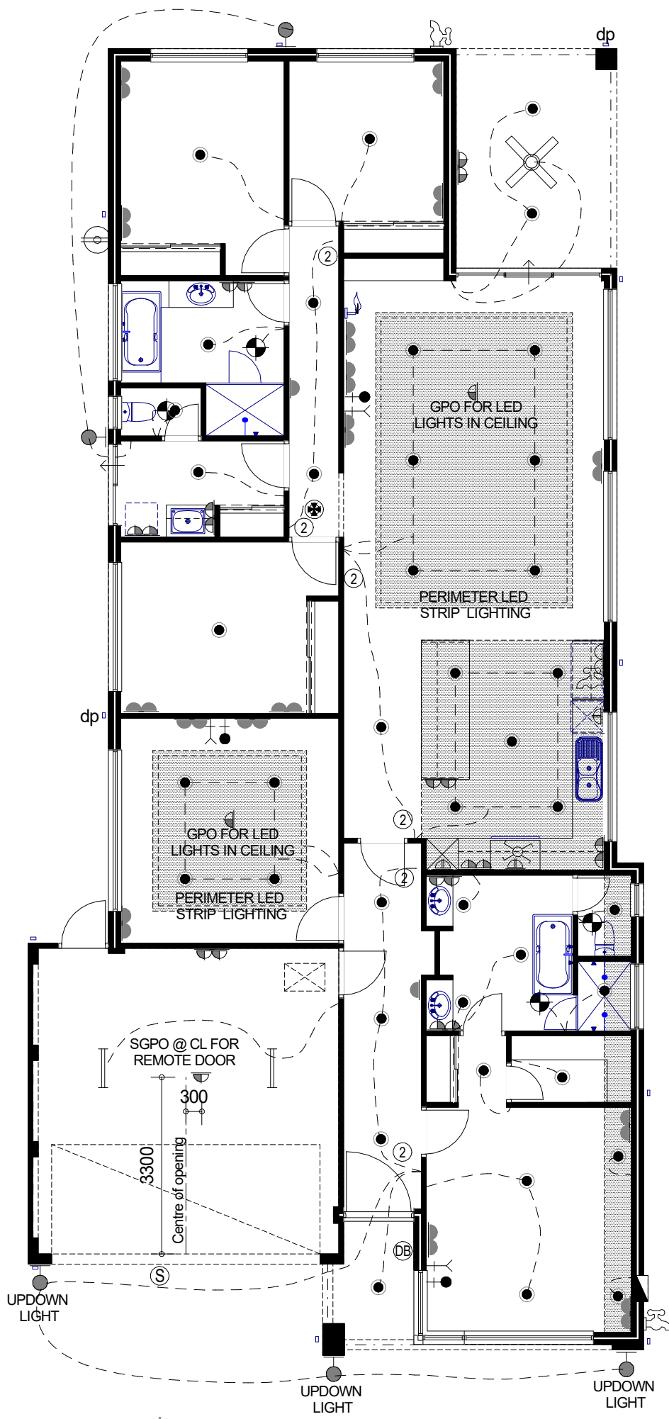
Electrical Plan Scale 1:100 @ A3
